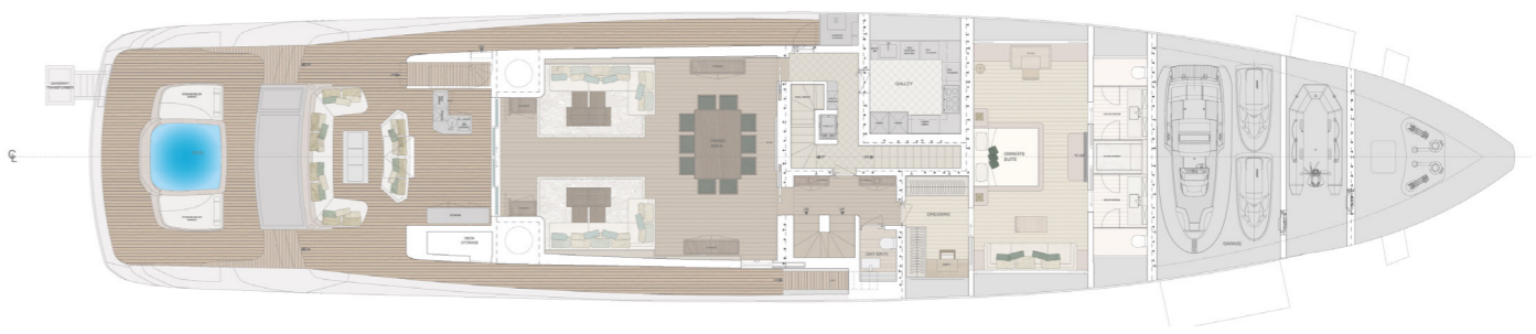
MAIN DECK
