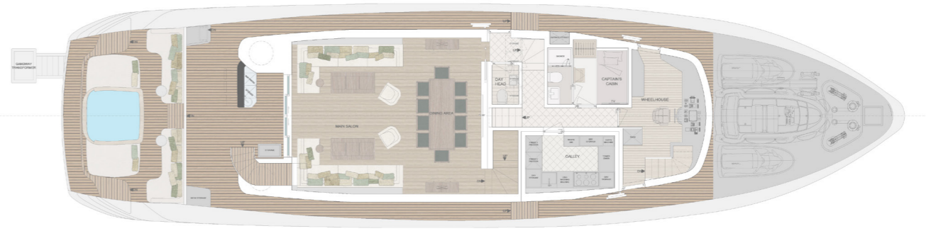
MAIN DECK \ BRIDGE DECK
